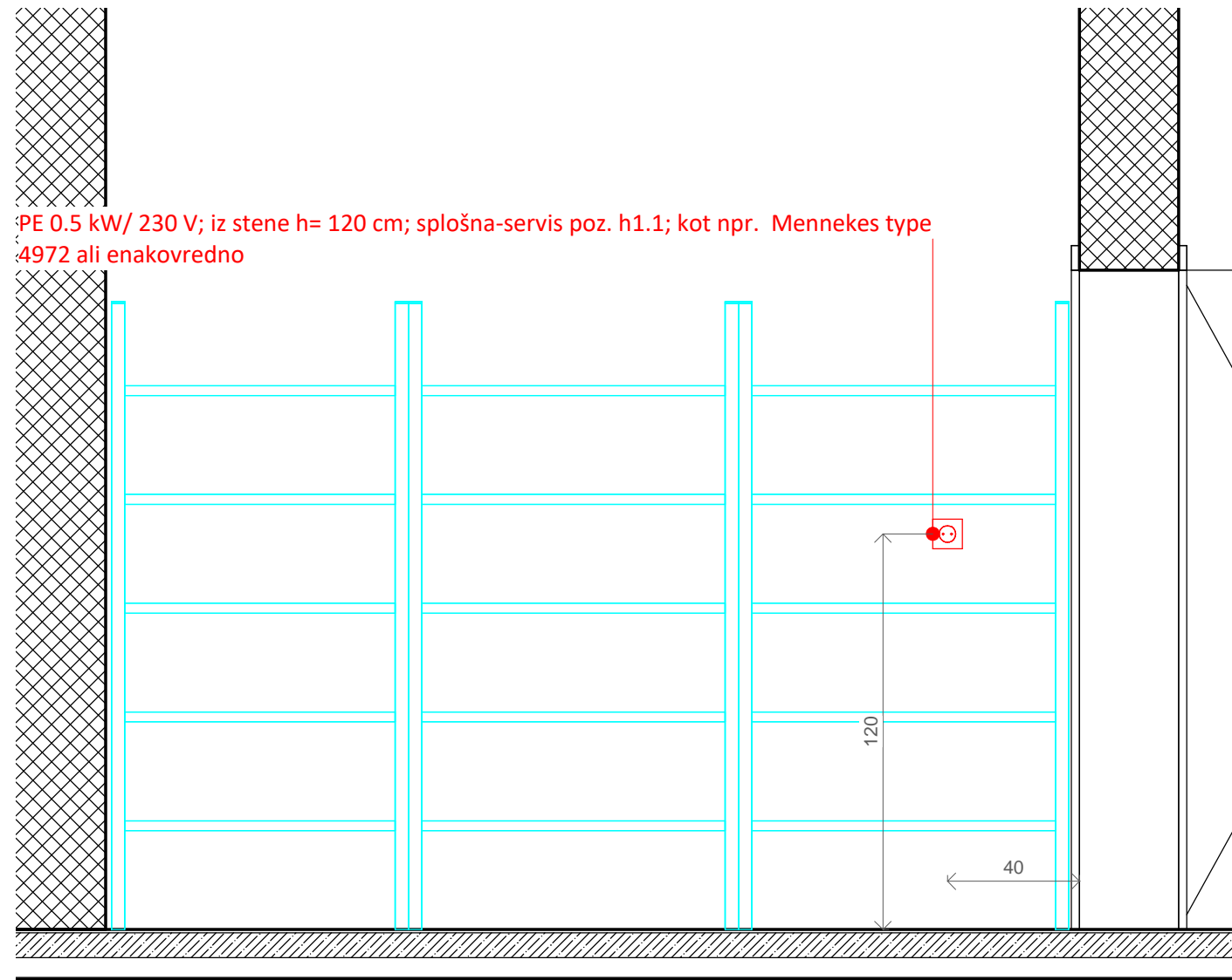
H - shramba gomoljnic M 1 : 20
