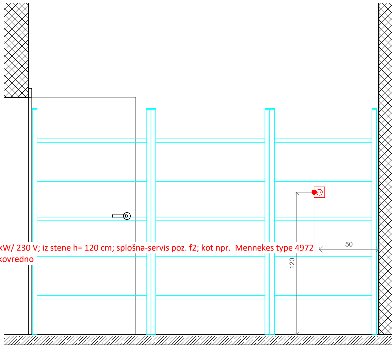
F - shramba suhih živil 2 M 1 : 20
