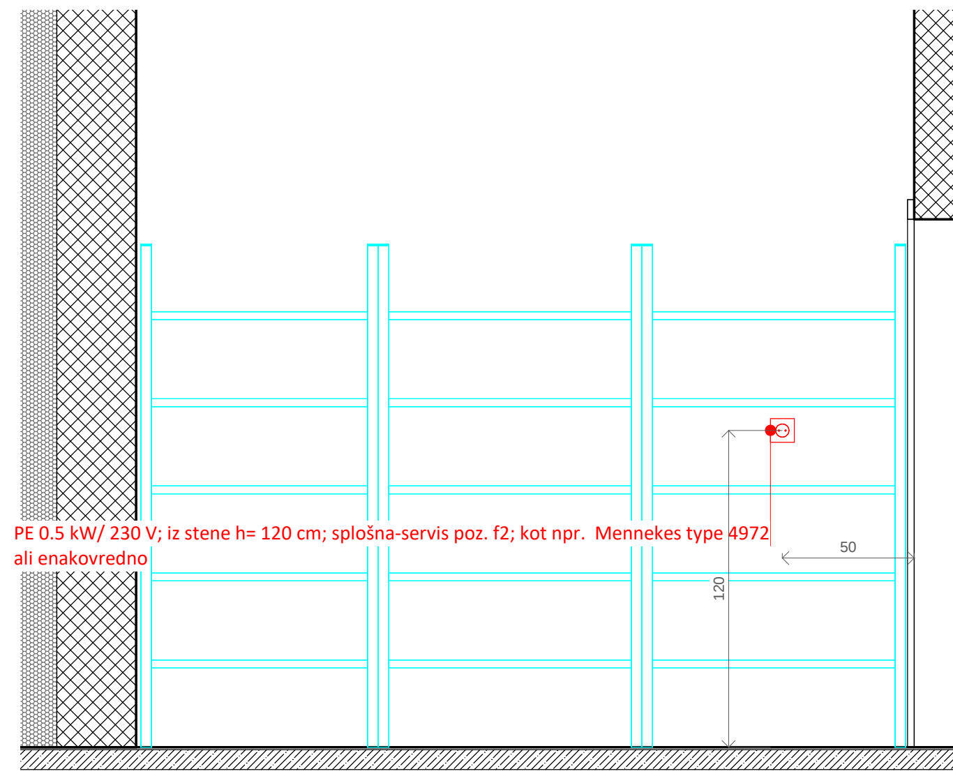
F - shramba suhih živil 1 M 1 : 20
