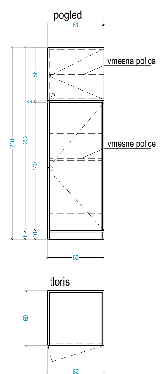
Poz.22 VISOKA OMARA 62/60, H=210cm pogled
